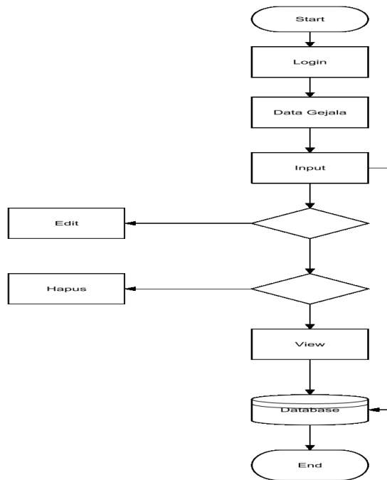
Gambar 2. Flowchart Admin
