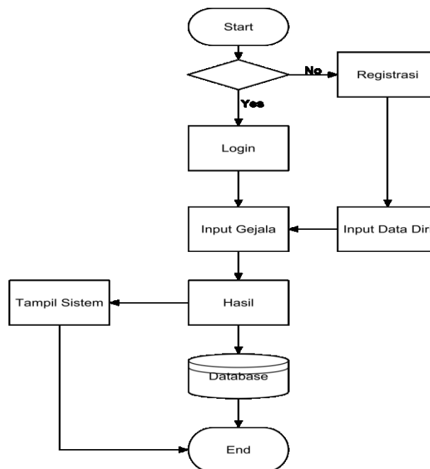
Gambar 1. Flowchart User
