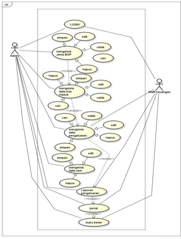
Gambar 3. Usecase Diagram
