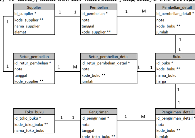
Gambar 4. Logical Record Structure
